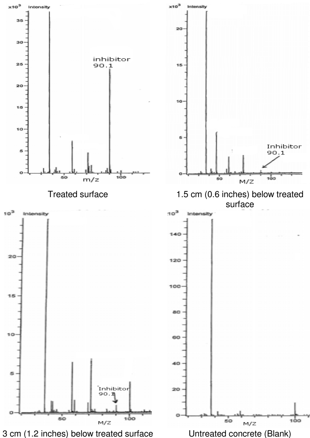
Figure 1 – Mass Spectra of Treatment A Coated Concrete at Various Depths
