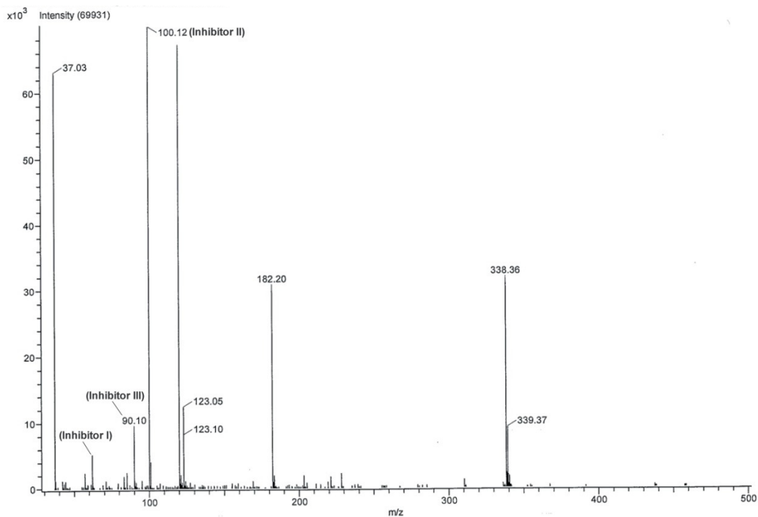
Figure 2.3 – Mass Spectrum of Concrete at 0.6 inches (1.5 cm) below Treated Surface
