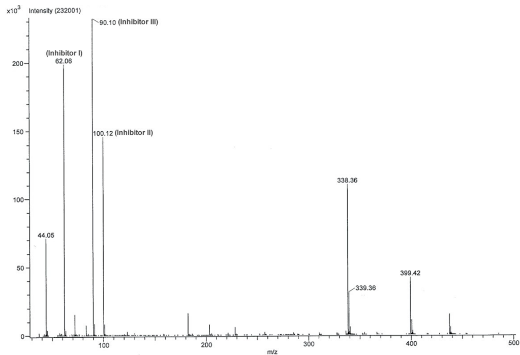
Figure 2.2 – Mass Spectrum of Concrete Surface of Treated Beam
