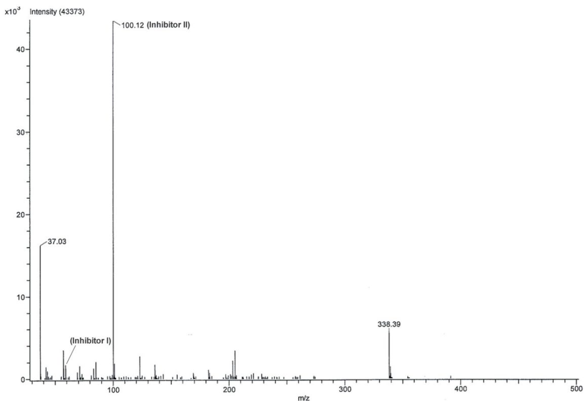
Figure 2.4 - Mass Spectrum of Concrete at 1.2 inches (3 cm) below Treated Surface
