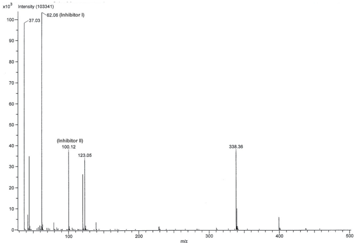
Figure 2.5 - Mass Spectrum of Concrete at 1.8 inches (4.8 cm) below Treated Surface
