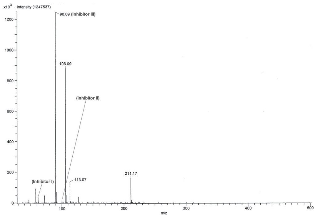
Figure 2.1 - Mass Spectrum of Treatment B
