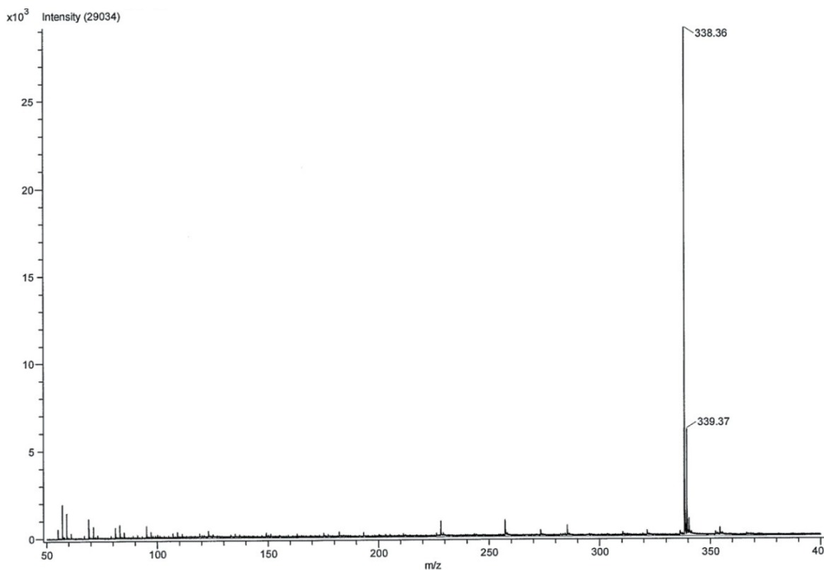
Figure 2.6 – Mass Spectrum of Untreated Concrete (control)
